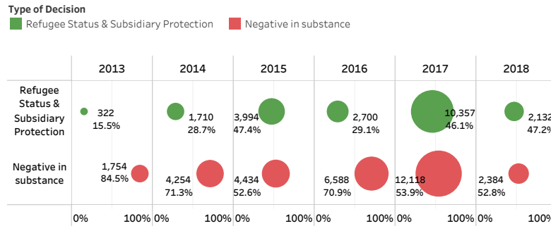
Recognition rate
