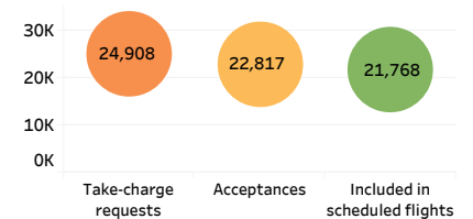
Relocation Procedures
